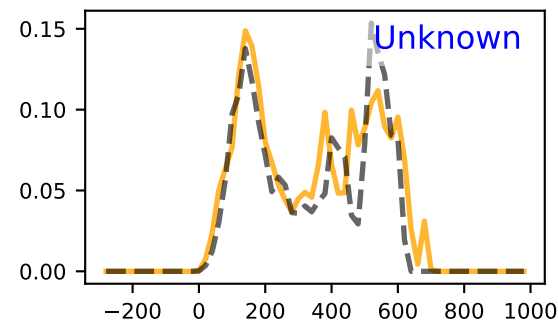
mp-560890
