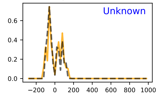
mp-8892
