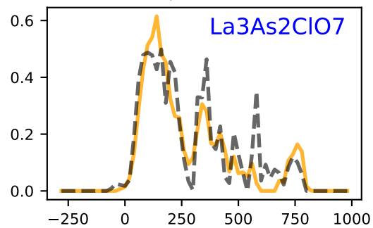
mp-28713
