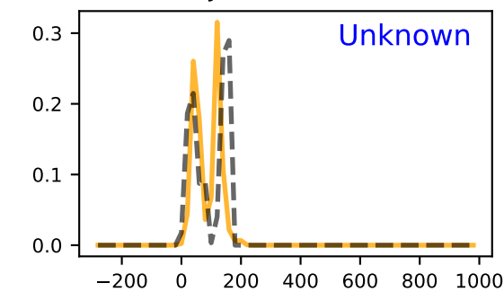
JVASP-19850
