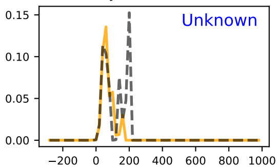
JVASP-68953
