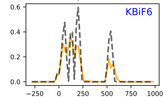
mp-555621
