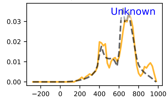
JVASP-15644
