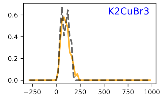
JVASP-67515
