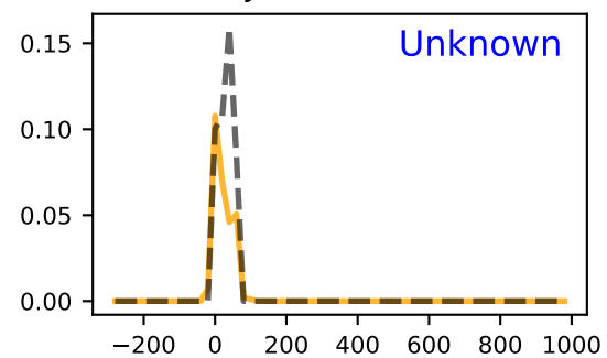
JVASP-15824
